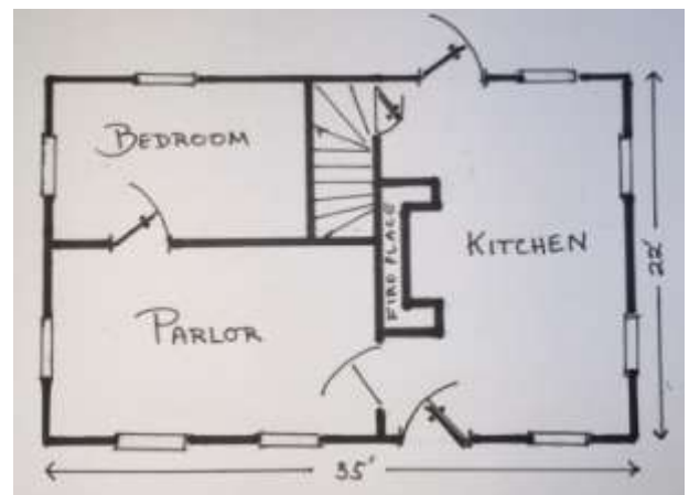
Fig. 2. A possible floor plan for Simon Jr's house. Drawing by M. Falconer.
